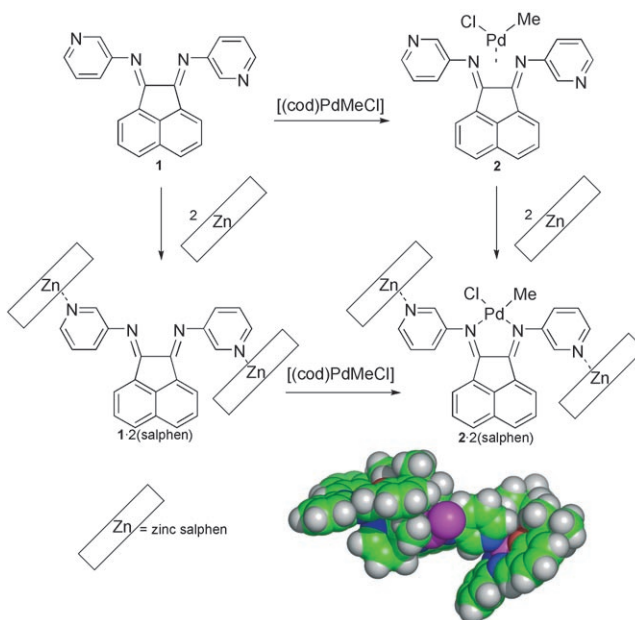
Scheme 2. Formation of an encapsulated neutral palladium complex and the PM3-TM optimized structure of the assembly with salphen C from Scheme 4; Pd, Zn, Cl all purple, O red, N blue, C green, H gray.
